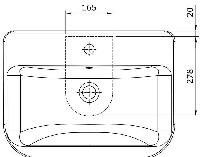
136340 - lavat.Look 60
