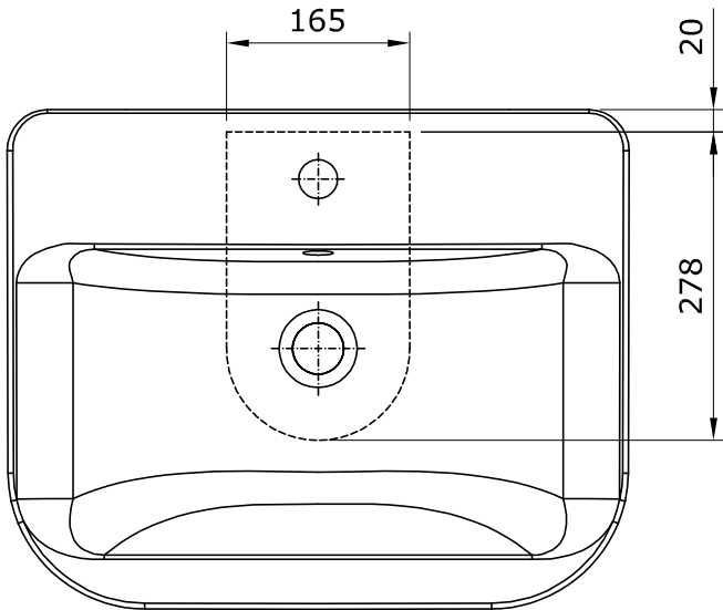
136330 - lavat.Look 56
