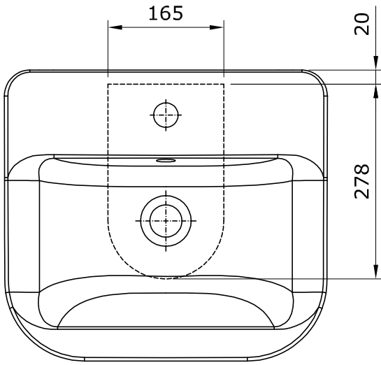
136310 - lavat.Look 46
