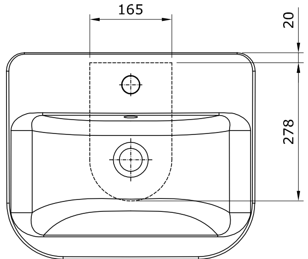
136320 - lavat.Look 50
